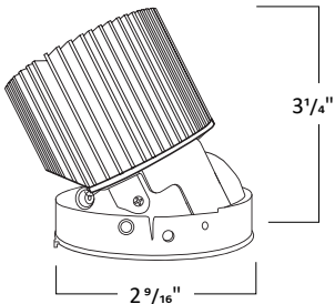
Module with tilted Heat Sink
