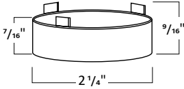
LED Holder (Head)
