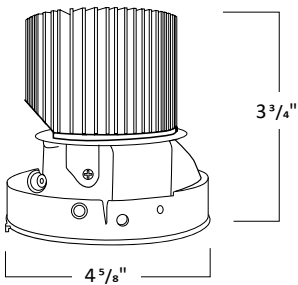
Module and Heat Sink
