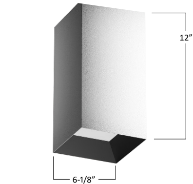
TRIM DIMENSIONS
