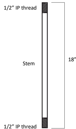
STEM MOUNT DIMENSION
