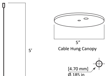
CABLE HUNG DIMENSION
